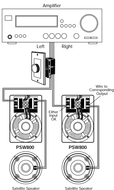
Figure 5 A Dual PSW800 Hook-Up
